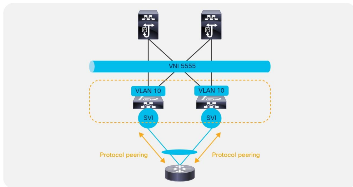
Figure 91 Dynamic routing: peering over vPC
