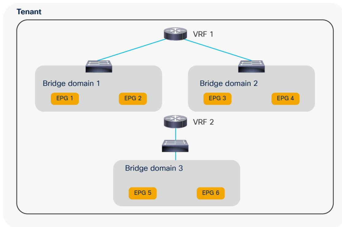
Figure 41 Hierarchy of tenants, private networks (VRF instances), bridge domains, and EPGs
