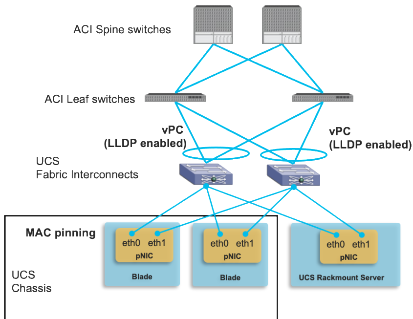
Figure 82 Cisco ACI leaf switches to UCS fabric interconnects connectivity
