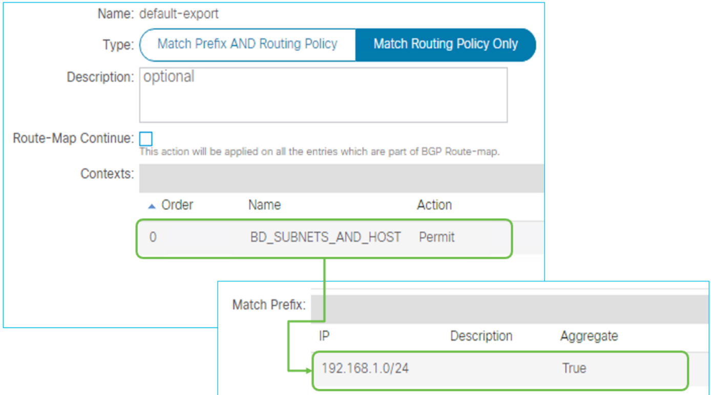
Figure 90 Route control for Host Route Advertisement
