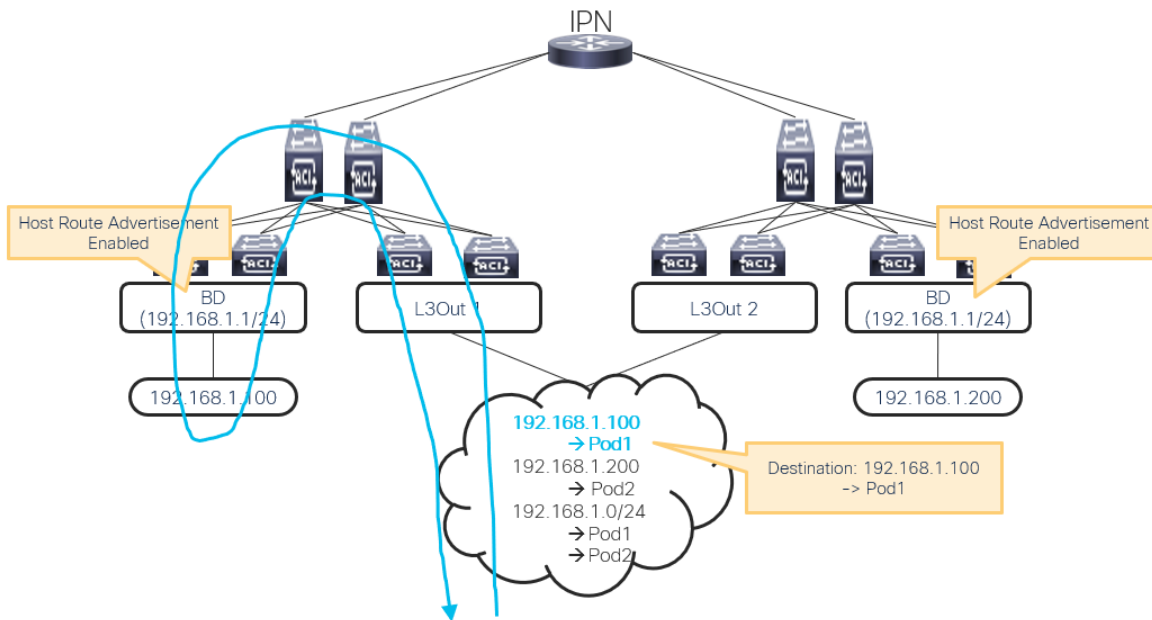
Figure 89 Efficient traffic flow with Host Route Advertisement
